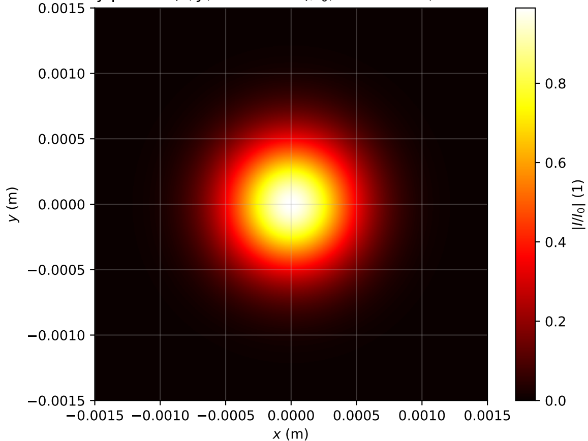
Intensity profile I(x, y, z = 0.637m)/I_0 , Pin=0.3Pcr, artificial time
